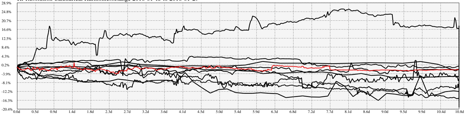
Hi-Resolution Calendrical Harmonics..Range 2016-01-15 to 2016-01-29
