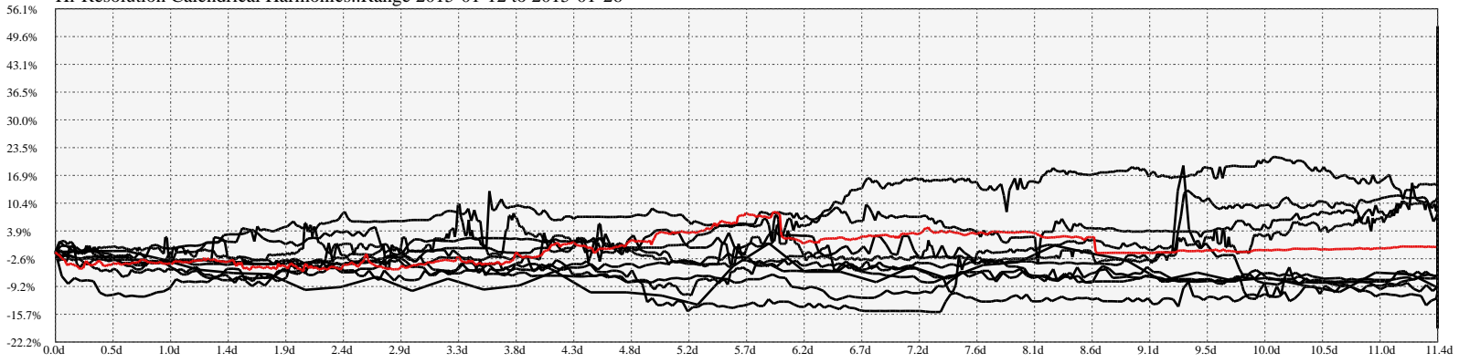
Hi-Resolution Calendrical Harmonics..Range 2015-01-12 to 2015-01-26
